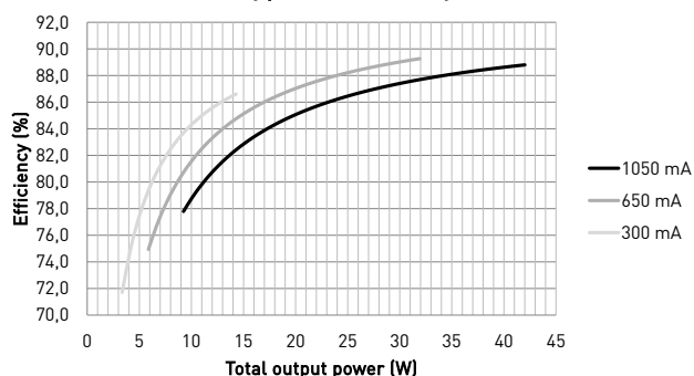
Typical efficiency
